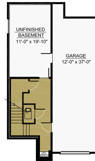
BASEMENT FLOOR PLAN-TUCK UNDER GARAGE
